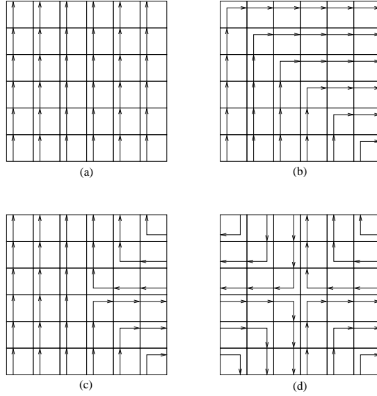
FIGURE 7. Exceptional points of X_k (uncolored)
