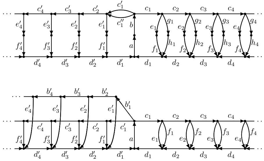
FIGURE 2. Pictured are the graph presentations of two locally compact countable state Markov shifts with very limited inner symmetry. The image of the canonical-boundary representation is thus fairly small within the group of all boundary-automorphisms.
